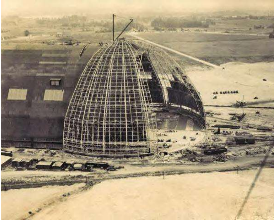
The clamshell doors are built on the Goodyear-Zeppelin Co.'s Airdock, in Akron, Ohio.
